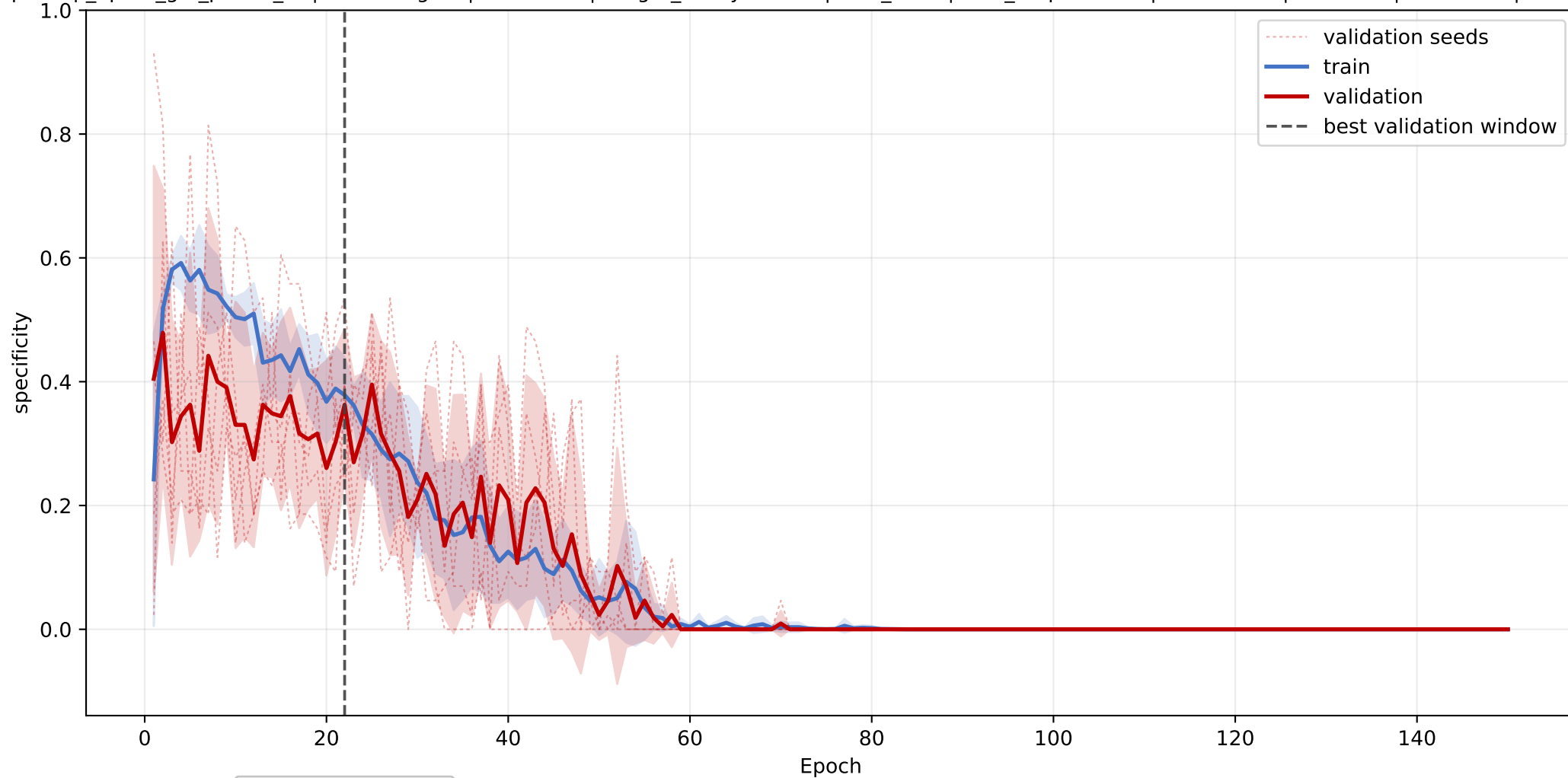
ML-scp2: mean specificity learning curve across seeds
