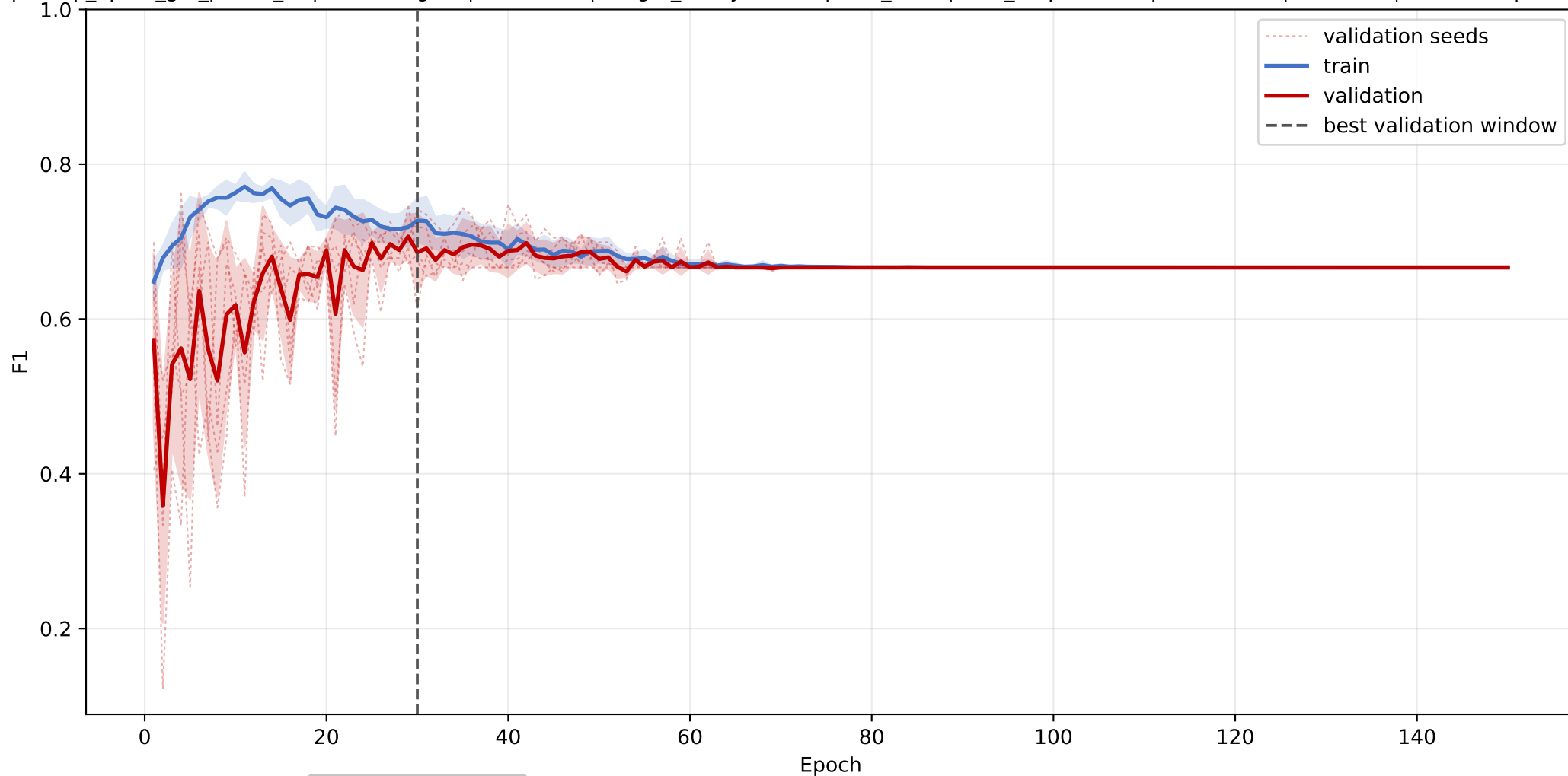
OSBP-scp2: mean F1 learning curve across seeds
