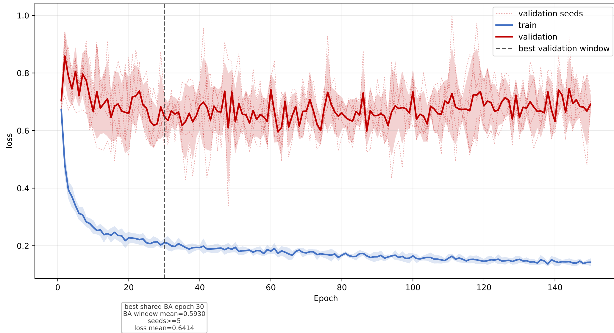
OSBP-scp2: mean loss learning curve across seeds
