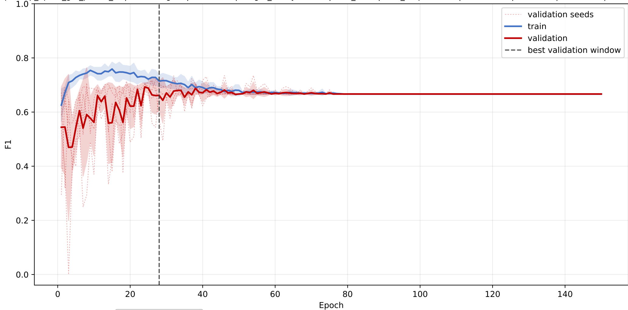
lipocalin-scp2: mean F1 learning curve across seeds
