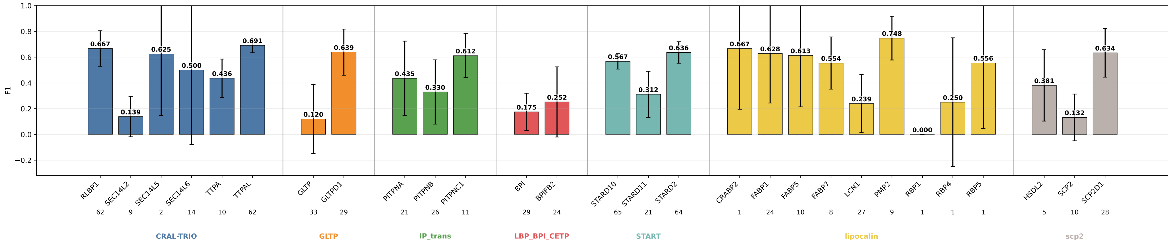
geometric_edge_mlp_protgeom8_no_buriedness_q50 F1 by subgroup geometric_edge_mlp_protgeom8_no_buriedness_q50 | class weights | lr=0.0001 | weight_decay=0.01 | final_m=4 | final_dropout=0.1 | hiddim=8 | heads=8 | batch=16 | ep=120 | seeds=0,1,2,3,4
