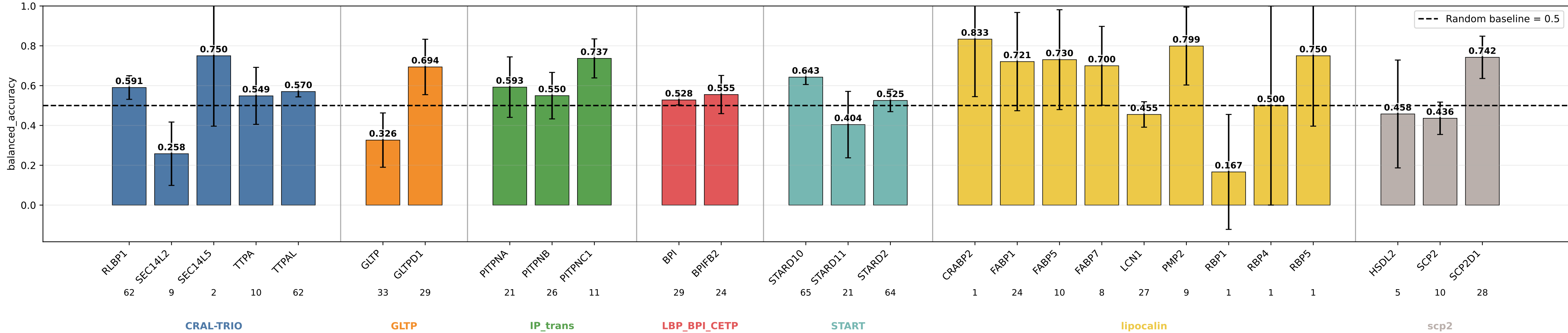
geometric_edge_mlp_protgeom8_no_buriedness_q50 balanced_accuracy by subgroup geometric_edge_mlp_protgeom8_no_buriedness_q50 | class weights | lr=0.0001 | weight_decay=0.01 | final_m=4 | final_dropout=0.1 | hiddim=8 | heads=8 | batch=16 | ep=120 | seeds=0,1,2,3,4
