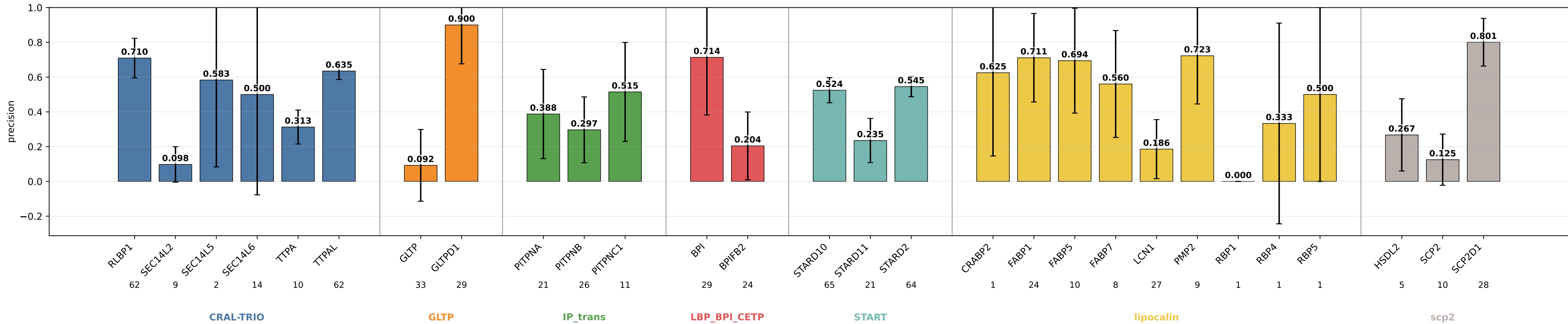
geometric_edge_mlp_protgeom8_no_buriedness_q50 precision by subgroup geometric_edge_mlp_protgeom8_no_buriedness_q50 | class weights | lr=0.0001 | weight_decay=0.01 | final_m=4 | final_dropout=0.1 | hiddim=8 | heads=8 | batch=16 | ep=120 | seeds=0,1,2,3,4
