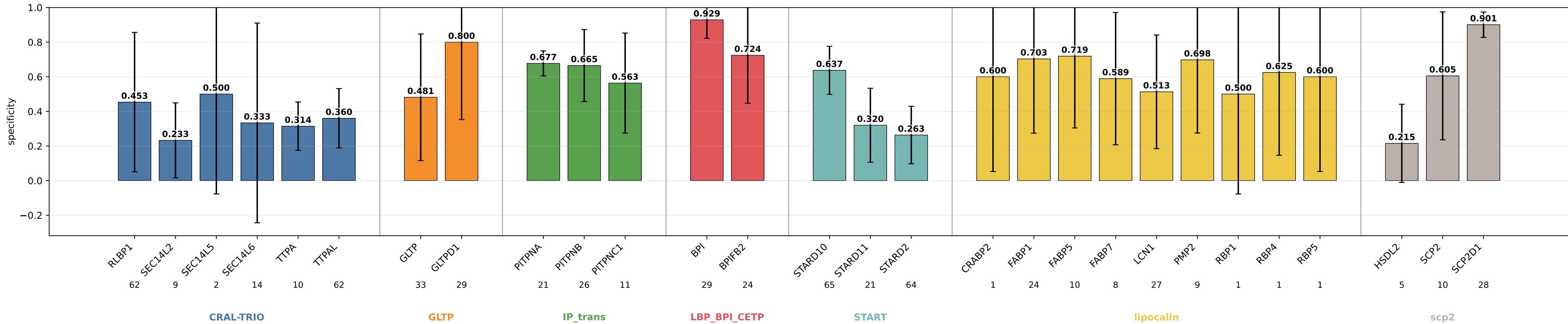
geometric_edge_mlp_protgeom8_no_buriedness_q50 specificity by subgroup geometric_edge_mlp_protgeom8_no_buriedness_q50 | class weights | lr=0.0001 | weight_decay=0.01 | final_m=4 | final_dropout=0.1 | hiddim=8 | heads=8 | batch=16 | ep=120 | seeds=0,1,2,3,4
