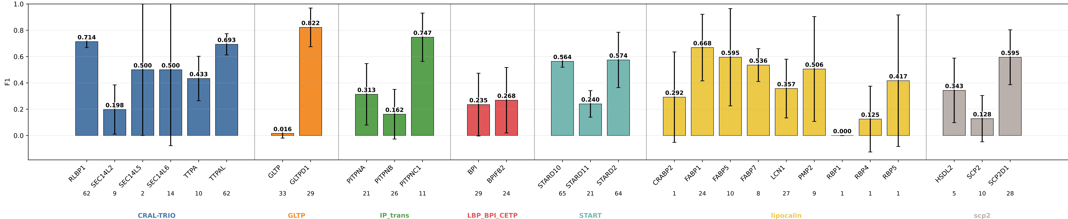
geometric_edge_mlp_protgeom8_no_depth_q10 F1 by subgroup geometric_edge_mlp_protgeom8_no_depth_q10 | class weights | lr=0.0001 | weight_decay=0.01 | final_m=4 | final_dropout=0.1 | hiddim=8 | heads=8 | batch=16 | ep=120 | seeds=0,1,2,3,4
