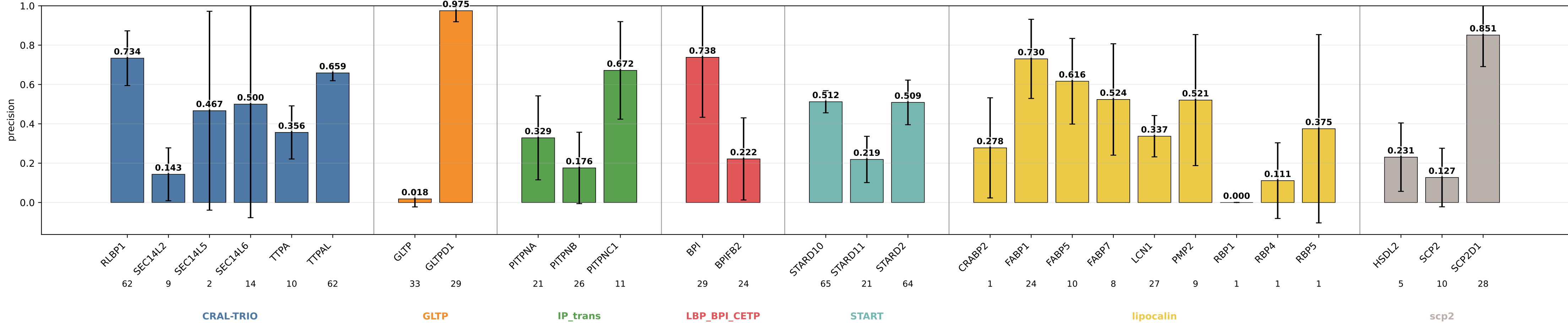
geometric_edge_mlp_protgeom8_no_depth_q10 precision by subgroup geometric_edge_mlp_protgeom8_no_depth_q10 | class weights | lr=0.0001 | weight_decay=0.01 | final_m=4 | final_dropout=0.1 | hiddim=8 | heads=8 | batch=16 | ep=120 | seeds=0,1,2,3,4
