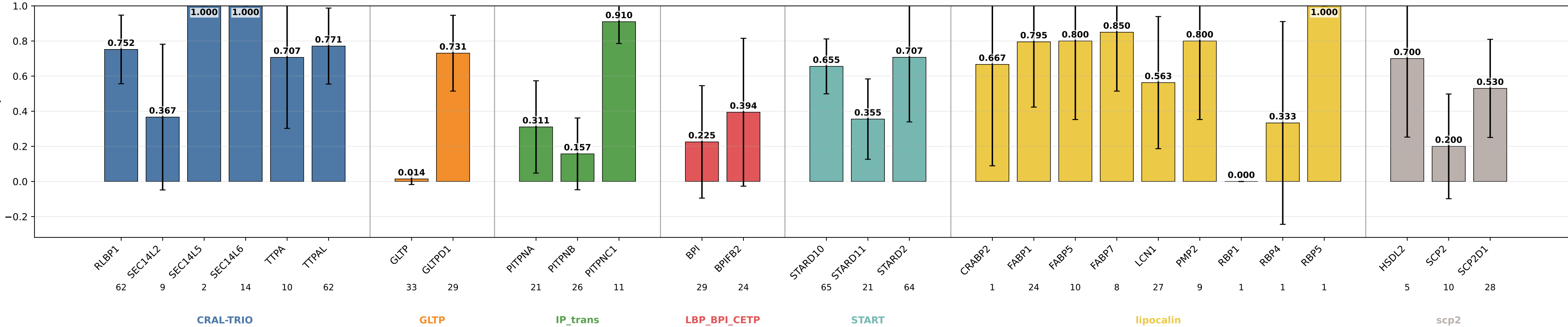
geometric_edge_mlp_protgeom8_no_depth_q10 sensitivity by subgroup geometric_edge_mlp_protgeom8_no_depth_q10 | class weights | lr=0.0001 | weight_decay=0.01 | final_m=4 | final_dropout=0.1 | hiddim=8 | heads=8 | batch=16 | ep=120 | seeds=0,1,2,3,4
