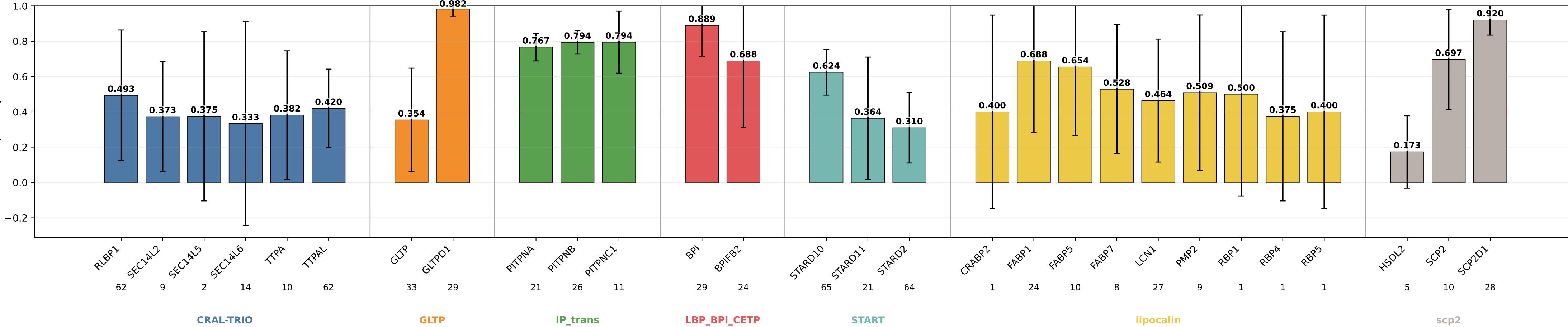
geometric_edge_mlp_protgeom8_no_depth_q10 specificity by subgroup geometric_edge_mlp_protgeom8_no_depth_q10 | class weights | lr=0.0001 | weight_decay=0.01 | final_m=4 | final_dropout=0.1 | hiddim=8 | heads=8 | batch=16 | ep=120 | seeds=0,1,2,3,4
