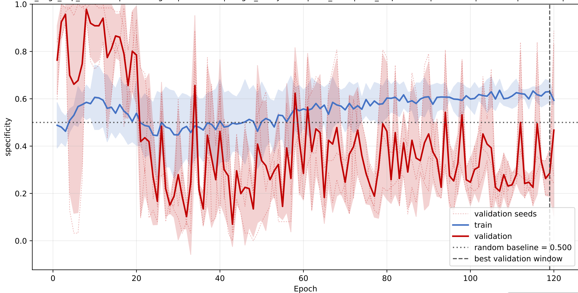
CRAL-TRIO: mean specificity learning curve across seeds
