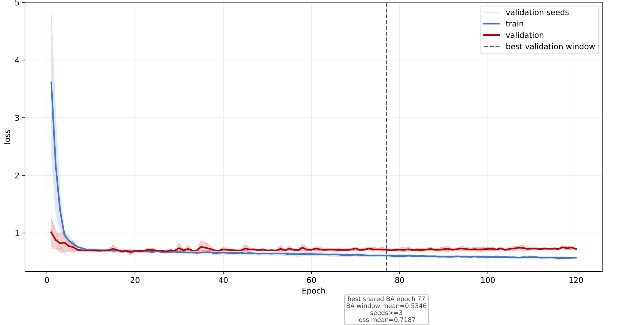
GLTP: mean loss learning curve across seeds
