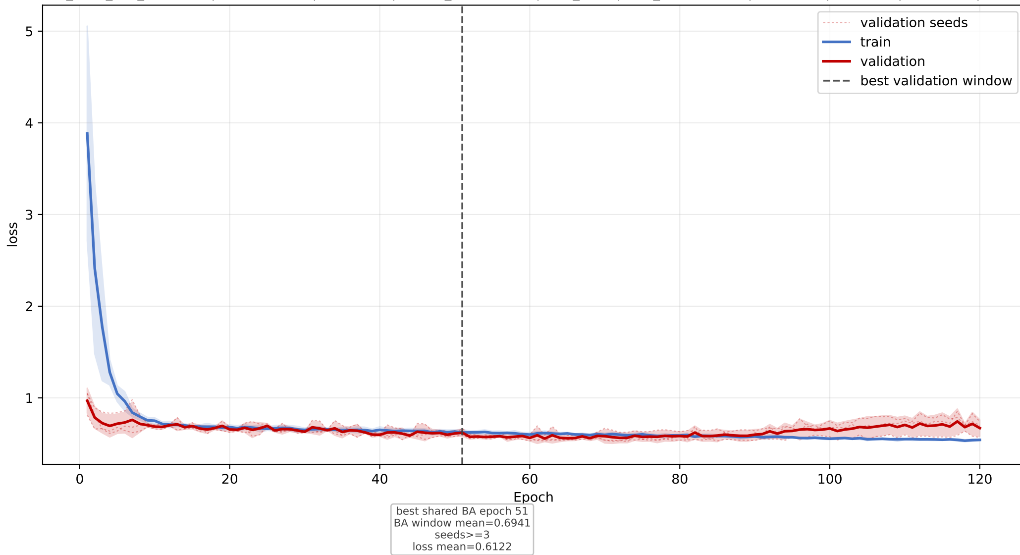
scp2: mean loss learning curve across seeds
