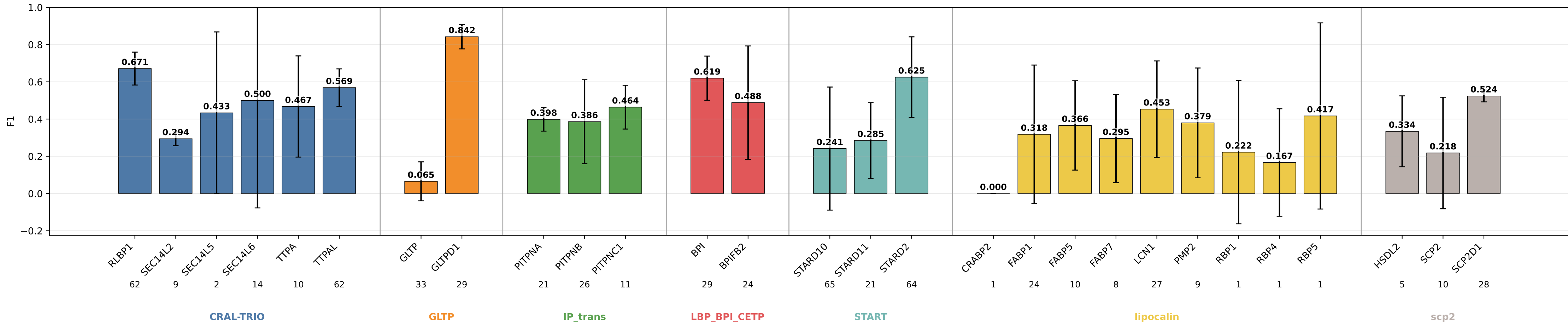
descriptors_head_family_neutral_lipprop F1 by subgroup descriptors_head_family_neutral_lipprop | class weights | lr=0.0001 | weight_decay=0.01 | final_m=4 | final_dropout=0.1 | hiddim=8 | heads=8 | batch=16 | ep=120 | seeds=0,1,2,3,4
