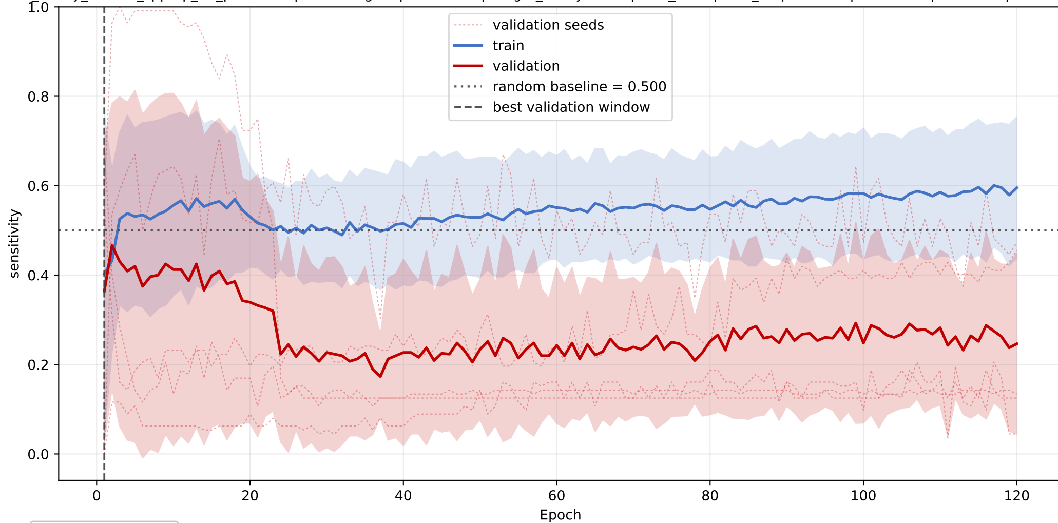
choline: mean sensitivity learning curve across seeds
