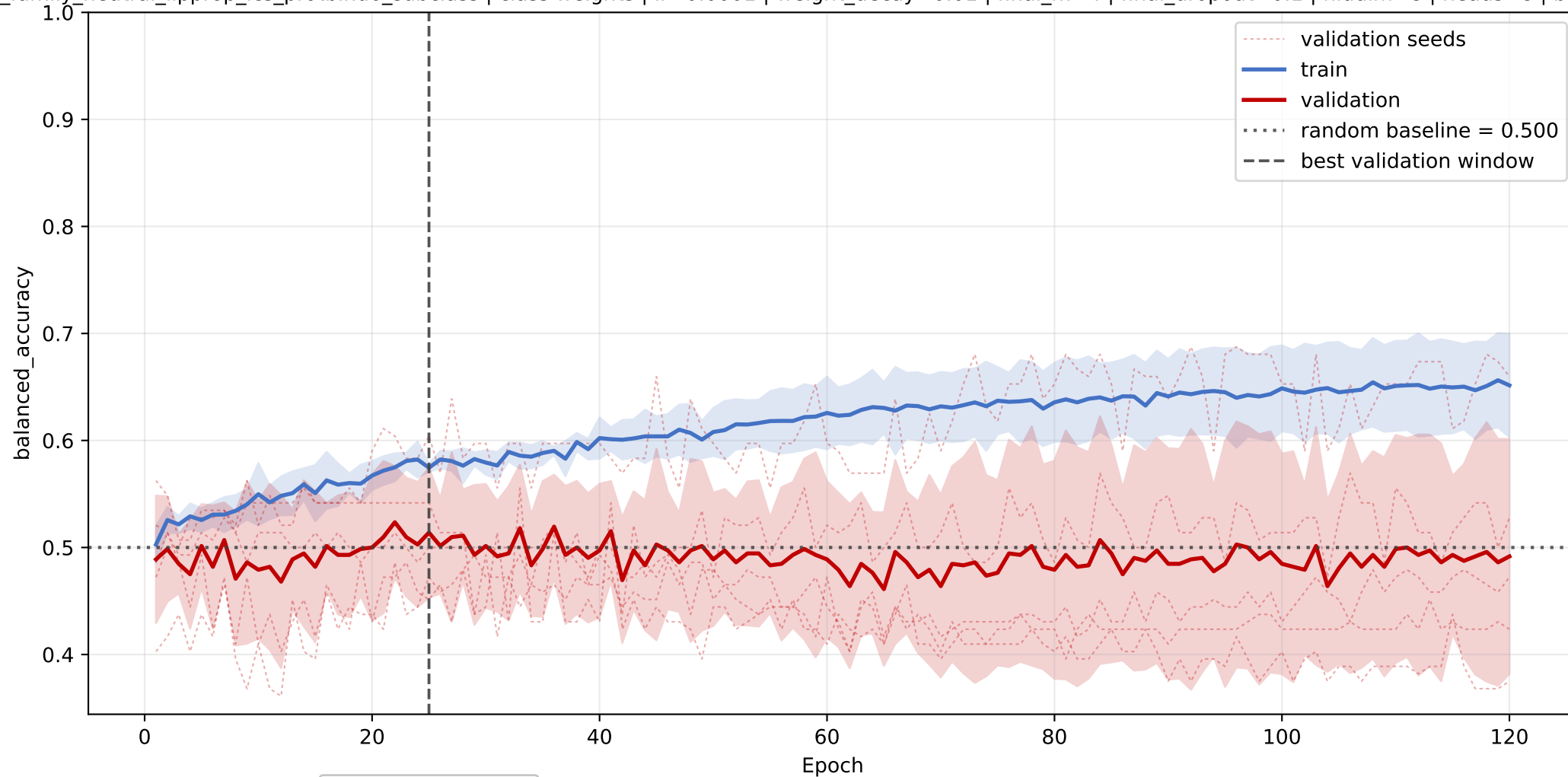
FA: mean balanced_accuracy learning curve across seeds
