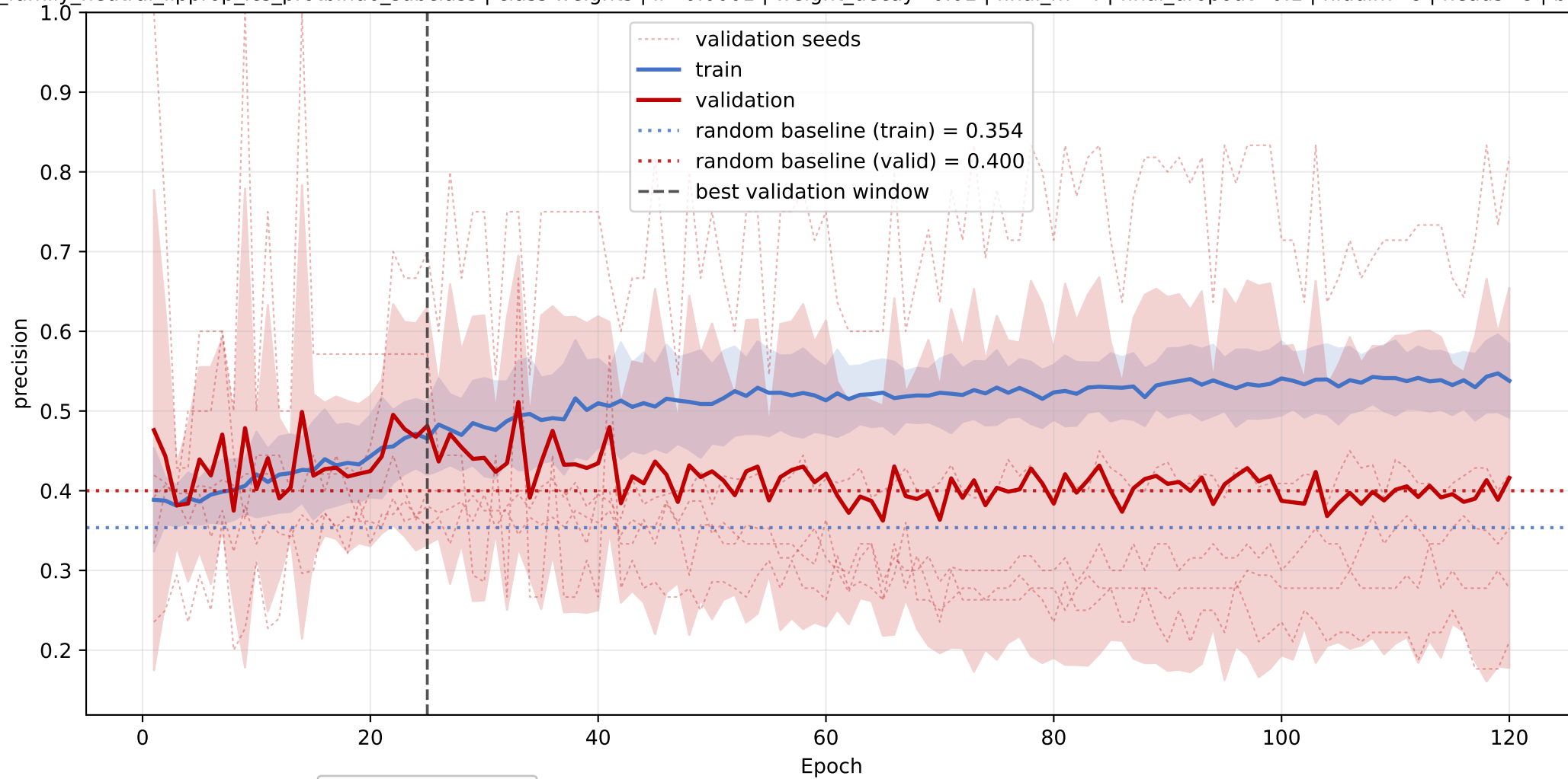
FA: mean precision learning curve across seeds
