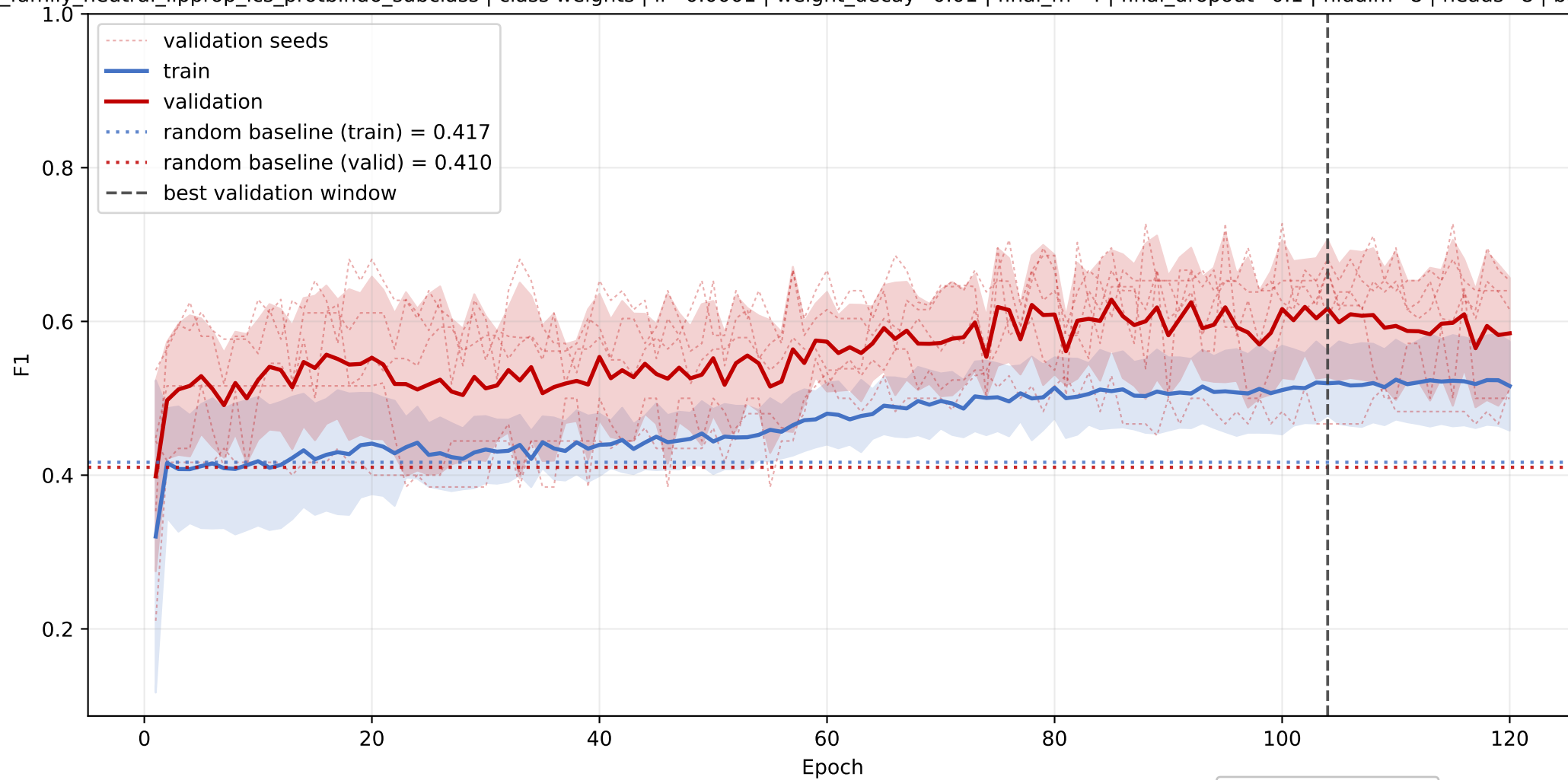
LPC+LPE+LPG: mean F1 learning curve across seeds
