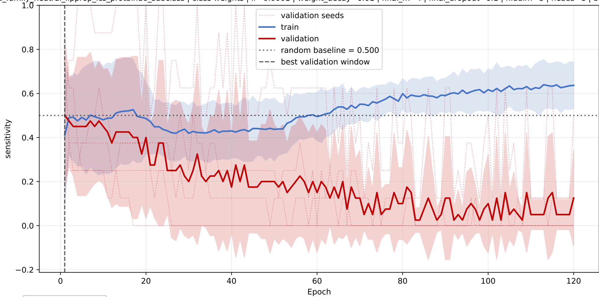
PI: mean sensitivity learning curve across seeds
