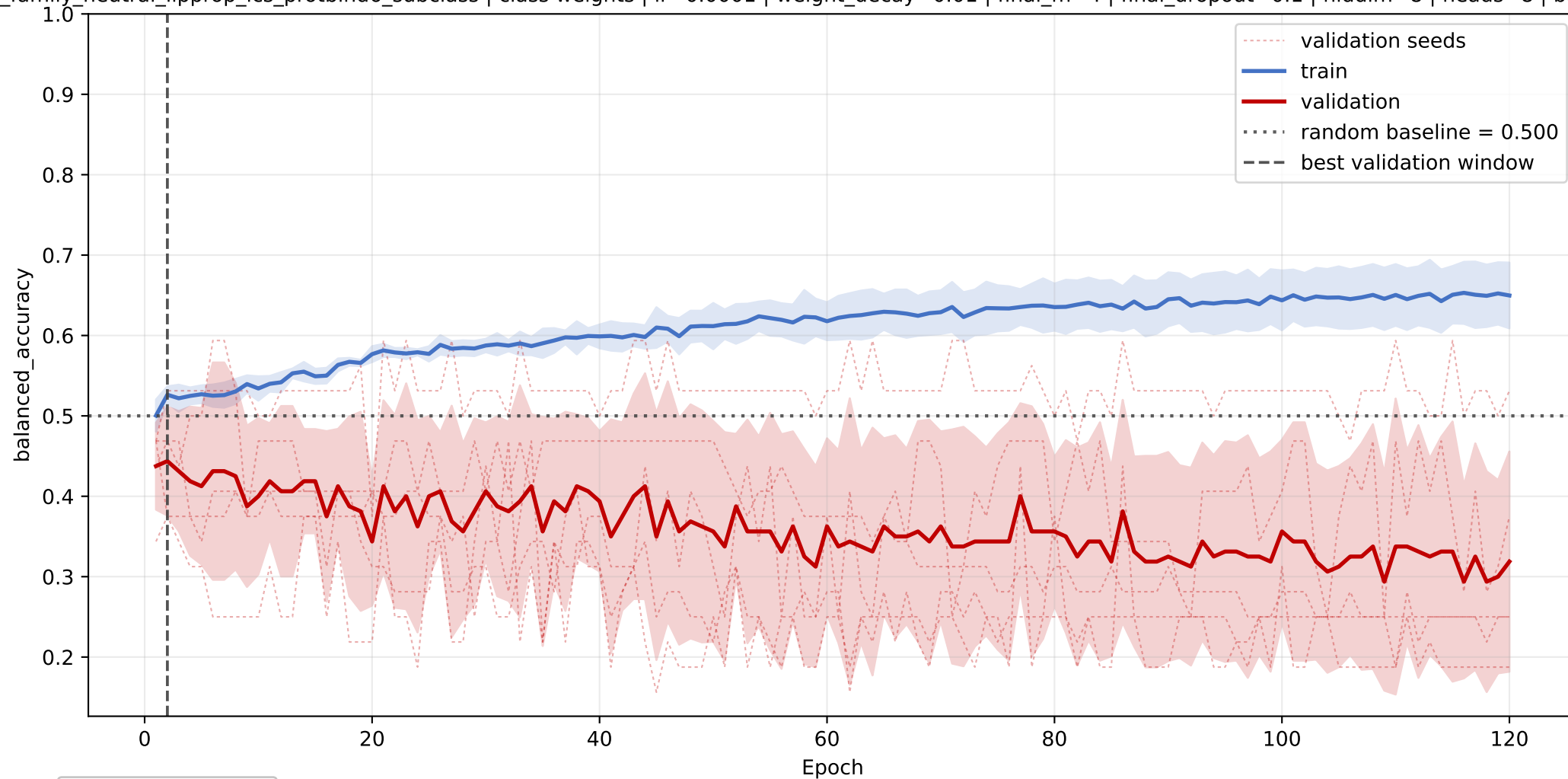
PS+PGP+DAG+TAG: mean balanced_accuracy learning curve across seeds
