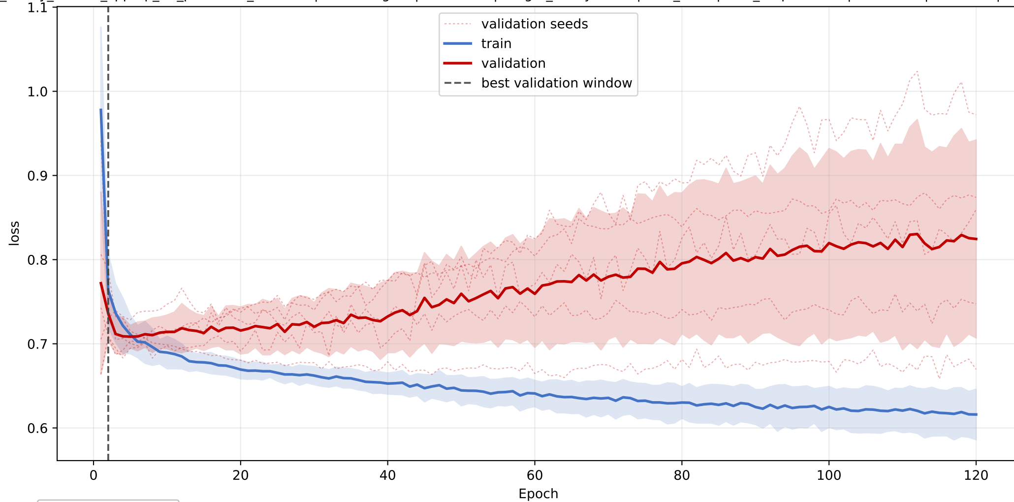
PS+PGP+DAG+TAG: mean loss learning curve across seeds
