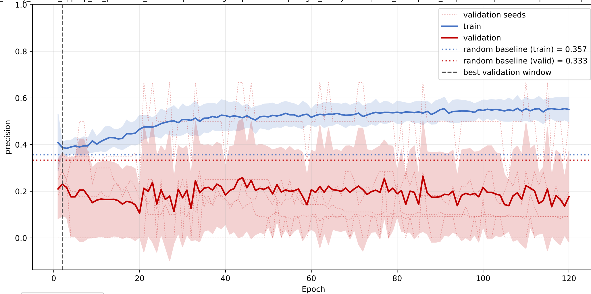
PS+PGP+DAG+TAG: mean precision learning curve across seeds
