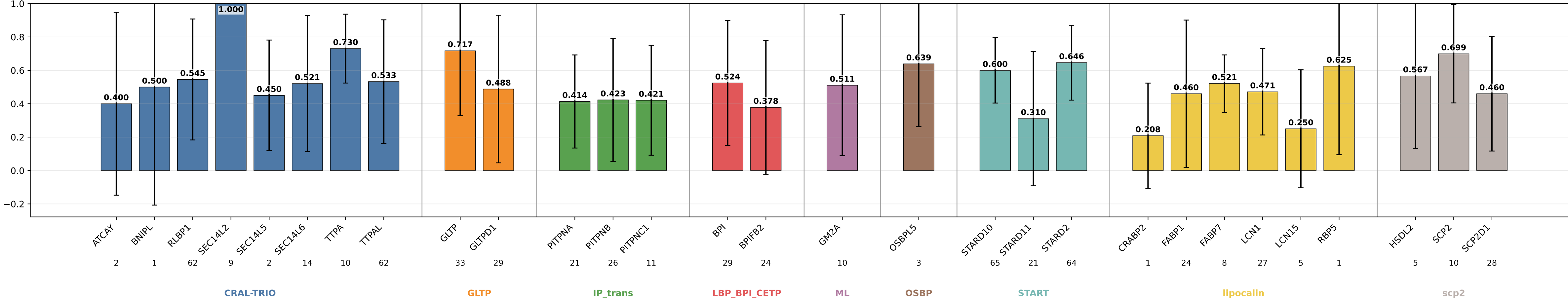
descriptors_head_family_neutral_lipprop_lcs_protbind6_subclass AUC by subgroup descriptors_head_family_neutral_lipprop_lcs_protbind6_subclass | class weights | lr=0.0001 | weight_decay=0.01 | final_m=4 | final_dropout=0.1 | hiddim=8 | heads=8 | batch=16 | ep=120 | seeds=0,1,2,3,4
