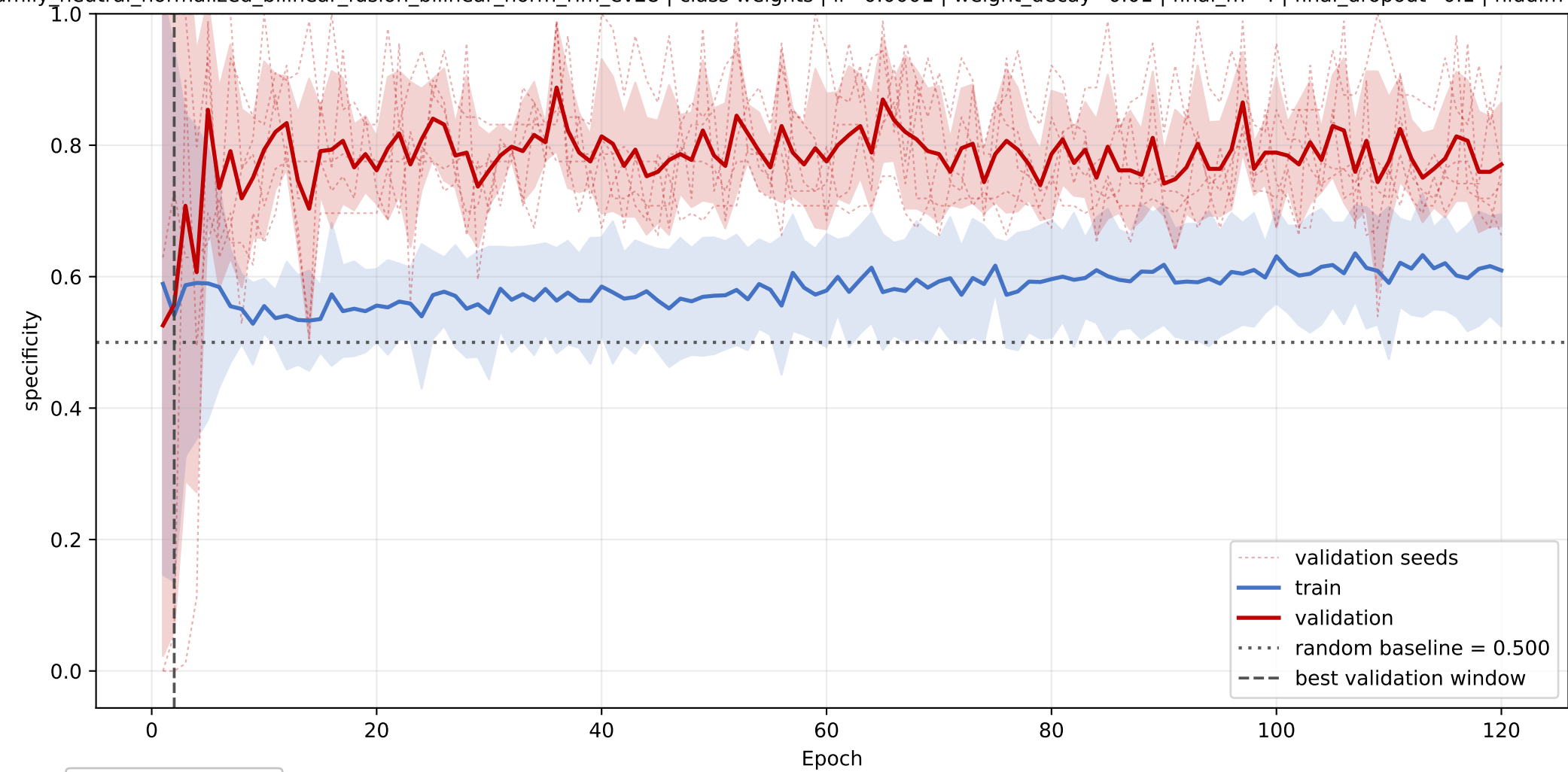
START: mean specificity learning curve across seeds
