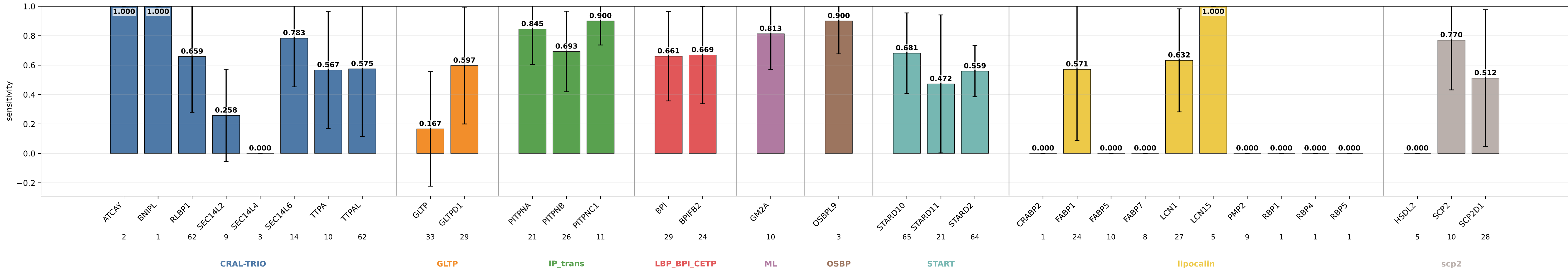
geometric_edge_mlp_protgeom_family_neutral_normalized_bilinear_fusion_bilinear_norm_lcs_esm3_balanced_lipid_classes_advprot sensitivity by subgroup geometric_edge_mlp_protgeom_family_neutral_normalized_bilinear_fusion_bilinear_norm_lcs_esm3_balanced_lipid_classes_advprot | class weights | lr=0.0001 | weight_decay=0.01 | final_m=4 | final_dropout=0.1 | hiddim=8 | heads=8 | batch=16 | ep=120 | seeds=0,1,2,3,4
