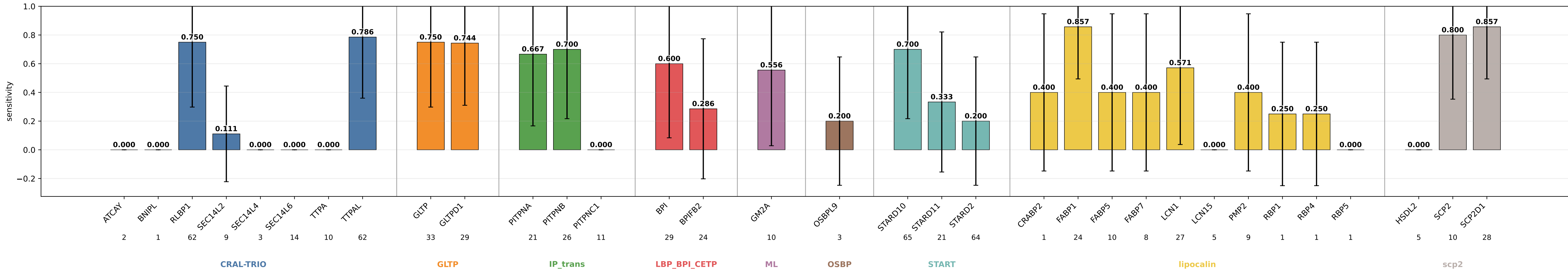
geometric_edge_mlp_protgeom_family_neutral_normalized_bilinear_fusion_bilinear_norm_lcs_esm3_balanced_lipid_classes_lipgraph sensitivity by subgroup geometric_edge_mlp_protgeom_family_neutral_normalized_bilinear_fusion_bilinear_norm_lcs_esm3_balanced_lipid_classes_lipgraph | class weights | lr=0.0001 | weight_decay=0.01 | final_m=4 | final_dropout=0.1 | hiddim=8 | heads=8 | batch=16 | ep=120 | seeds=0,1,2,3,4
