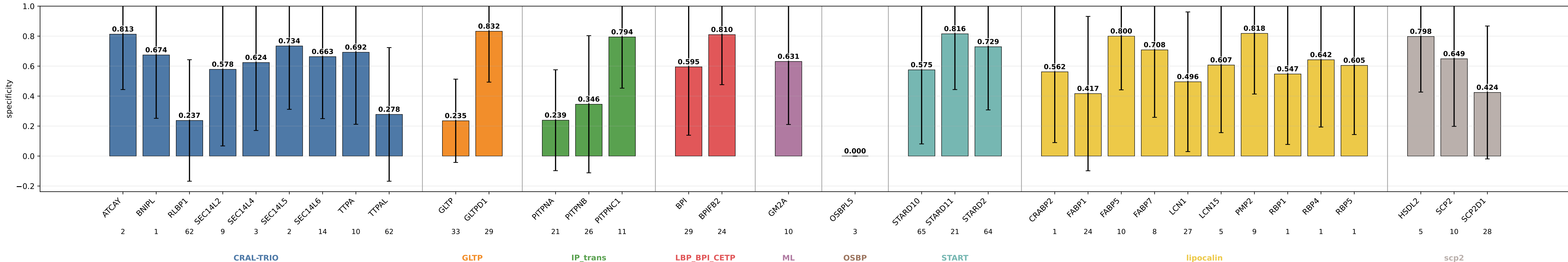
geometric_edge_mlp_protgeom_family_neutral_normalized_bilinear_fusion_bilinear_norm_lcs_esm3_balanced_lipid_classes_lipid64 specificity by subgroup geometric_edge_mlp_protgeom_family_neutral_normalized_bilinear_fusion_bilinear_norm_lcs_esm3_balanced_lipid_classes_lipid64 | class weights | lr=0.0001 | weight_decay=0.01 | final_m=4 | final_dropout=0.1 | hiddim=8 | heads=8 | batch=16 | ep=120 | seeds=0,1,2,3,4
