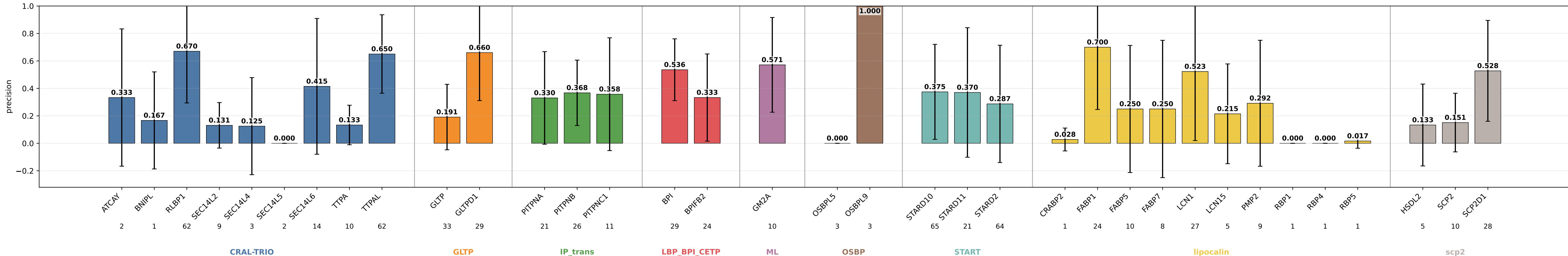
geometric_edge_mlp_protgeom_family_neutral_normalized_bilinear_fusion_bilinear_norm_lcs_esm3_balanced_lipid_classes_rankprot_advprot precision by subgroup geometric_edge_mlp_protgeom_family_neutral_normalized_bilinear_fusion_bilinear_norm_lcs_esm3_balanced_lipid_classes_rankprot_advprot | class weights | lr=0.0001 | weight_decay=0.01 | final_m=4 | final_dropout=0.1 | hiddim=8 | heads=8 | batch=64 | ep=120 | seeds=0,1,2,3,4
