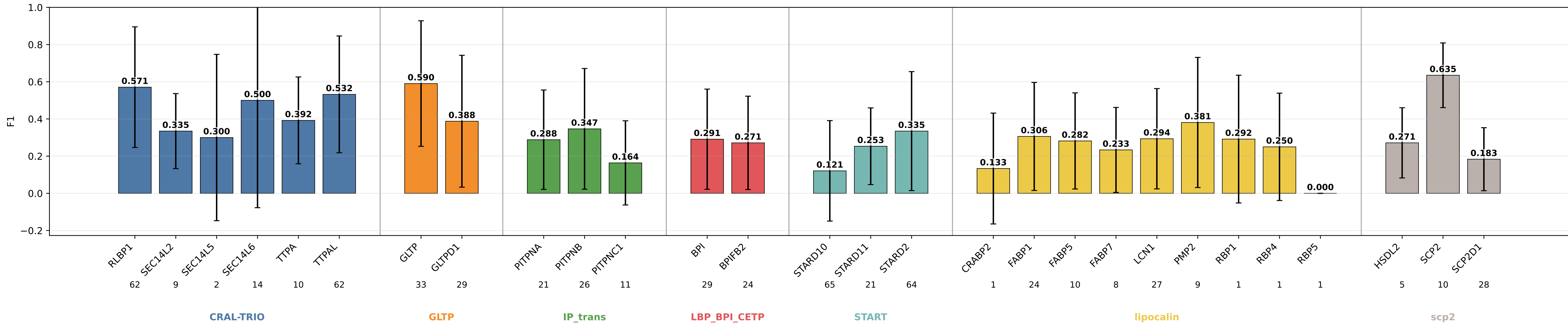
descriptors_pair_only_rankprot F1 by subgroup descriptors_pair_only_rankprot | class weights | lr=0.0001 | weight_decay=0.01 | final_m=4 | final_dropout=0.1 | hiddim=8 | heads=8 | batch=32 | ep=120 | seeds=0,1,2,3,4
