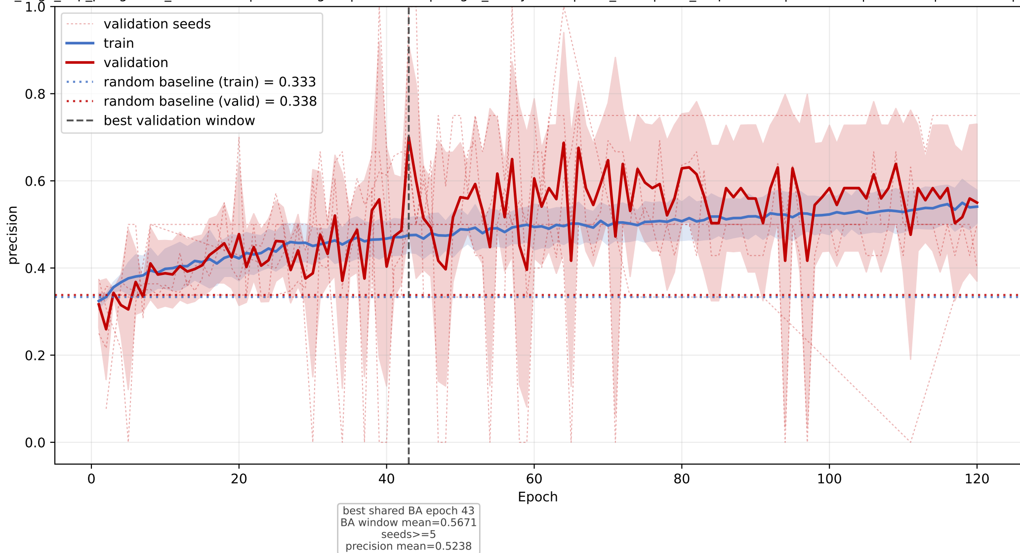
LBP_BPI_CETP: mean precision learning curve across seeds
