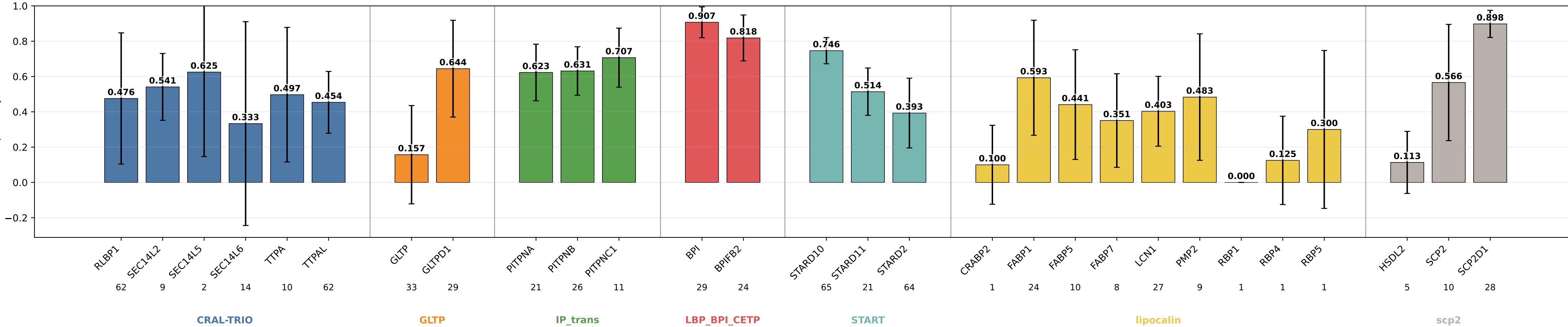
geometric_edge_mlp_protgeom8_normalized specificity by subgroup geometric_edge_mlp_protgeom8_normalized | class weights | lr=0.0001 | weight_decay=0.01 | final_m=4 | final_dropout=0.1 | hiddim=8 | heads=8 | batch=16 | ep=120 | seeds=0,1,2,3,4
