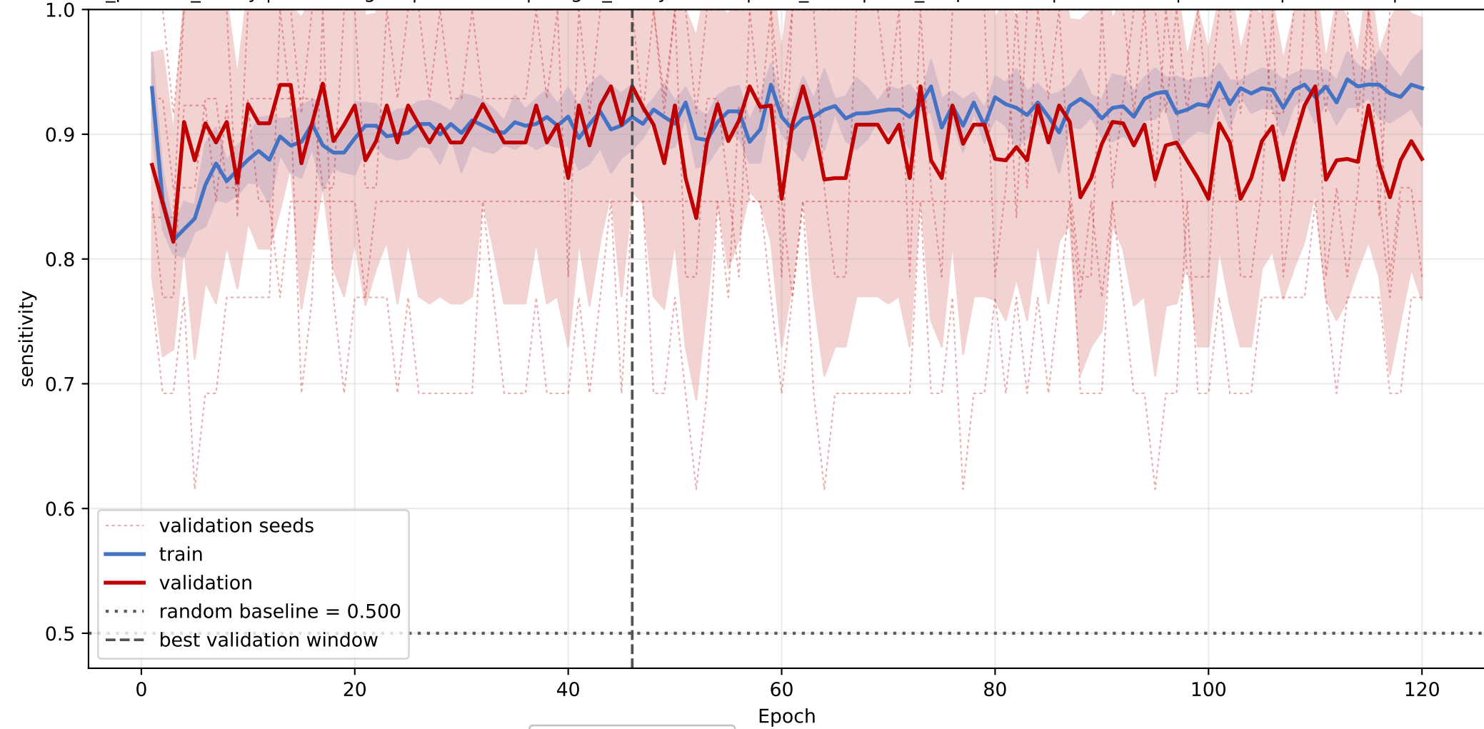
CRAL-TRIO: mean sensitivity learning curve across seeds
