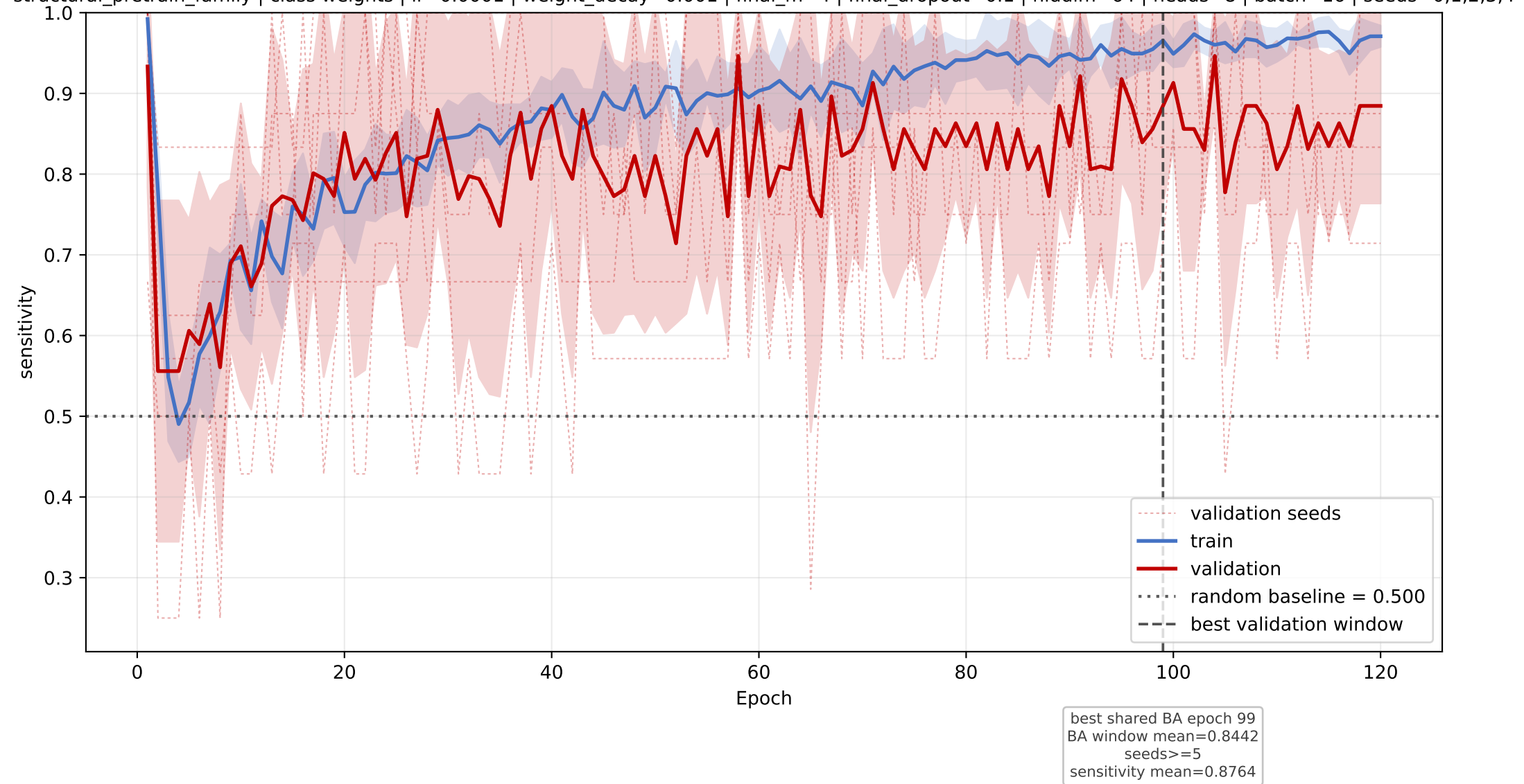
lipocalin: mean sensitivity learning curve across seeds
