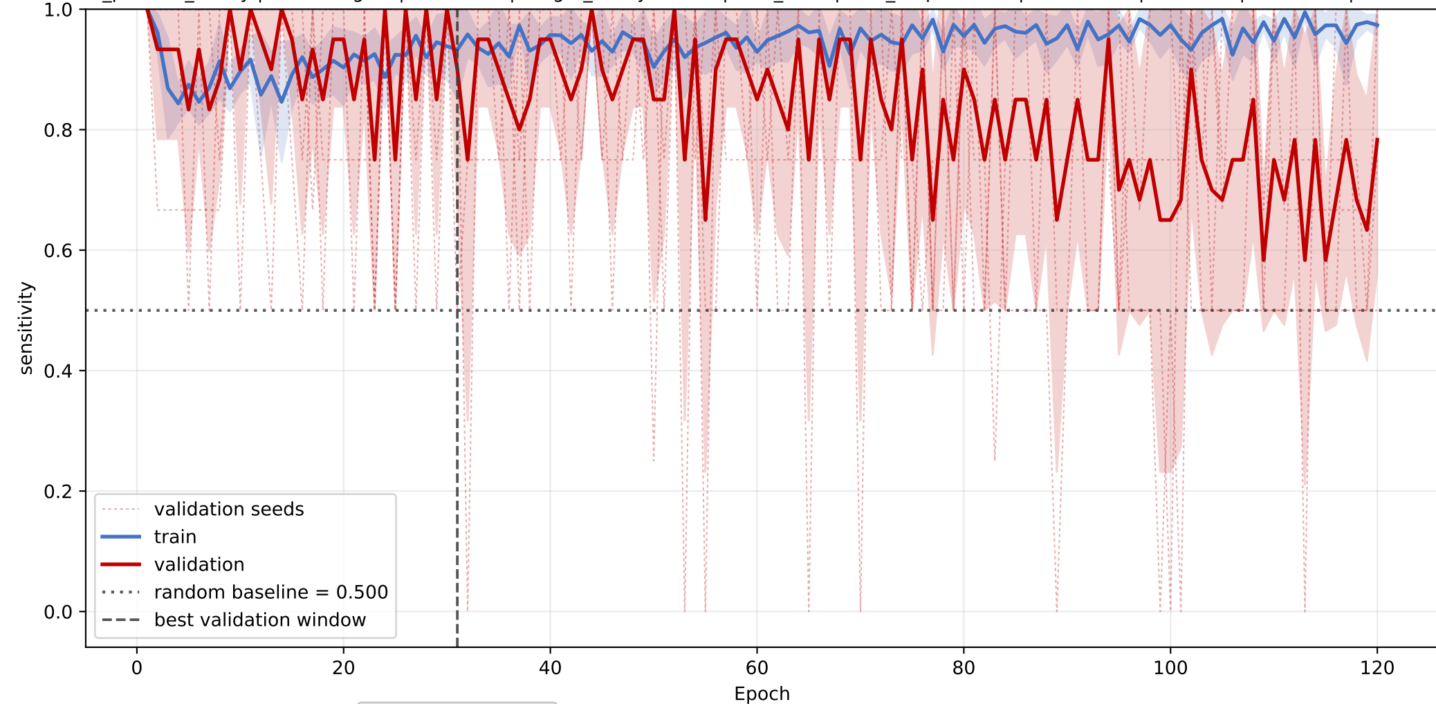
scp2: mean sensitivity learning curve across seeds
