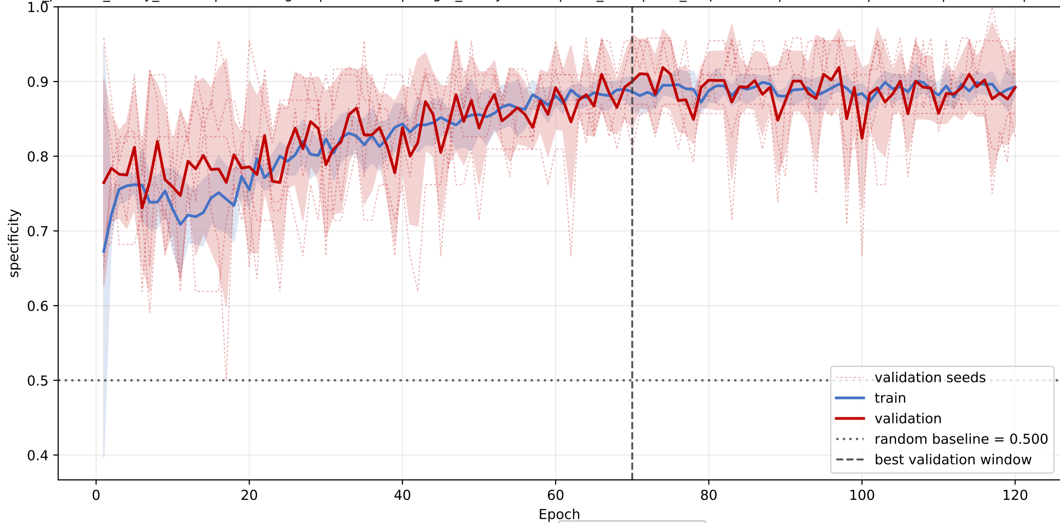
START: mean specificity learning curve across seeds
