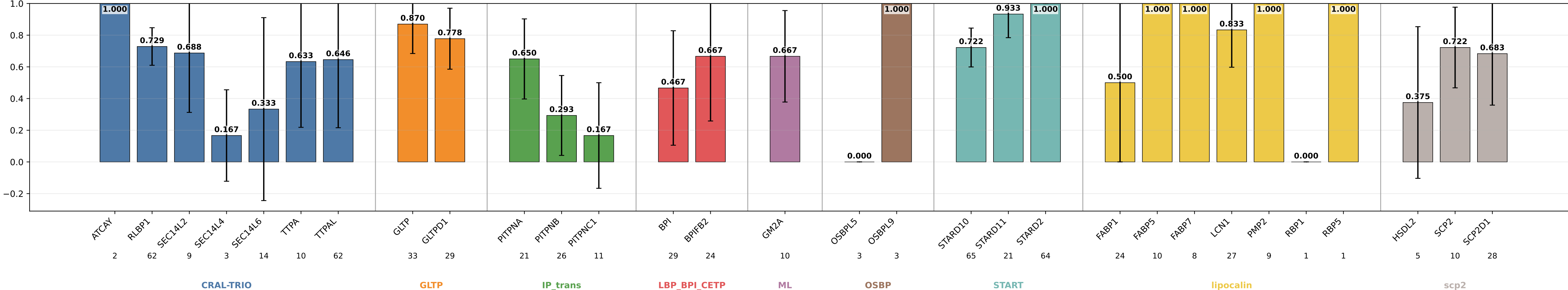
structural_pretrain_family_scratch precision by subgroup structural_pretrain_family_scratch | class weights | lr=0.0001 | weight_decay=0.001 | final_m=4 | final_dropout=0.1 | hiddim=64 | heads=8 | batch=16 | ep=120 | seeds=0,1,2,3,4
