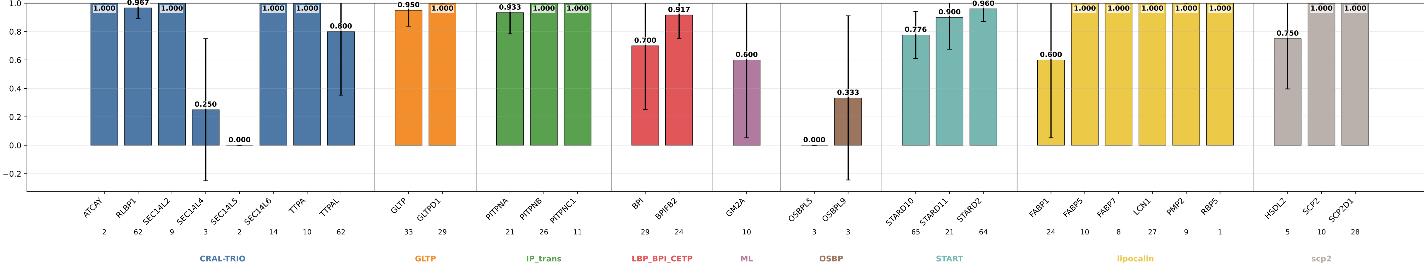
structural_pretrain_family_scratch sensitivity by subgroup structural_pretrain_family_scratch | class weights | lr=0.0001 | weight_decay=0.001 | final_m=4 | final_dropout=0.1 | hiddim=64 | heads=8 | batch=16 | ep=120 | seeds=0,1,2,3,4
