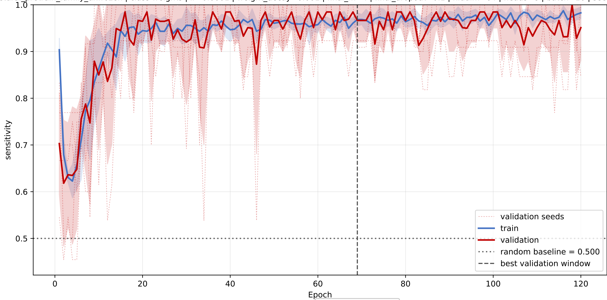
START: mean sensitivity learning curve across seeds
