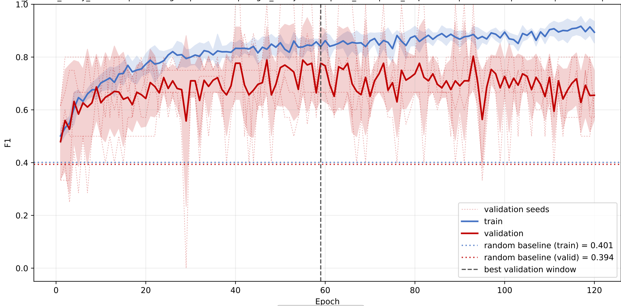
scp2: mean F1 learning curve across seeds
