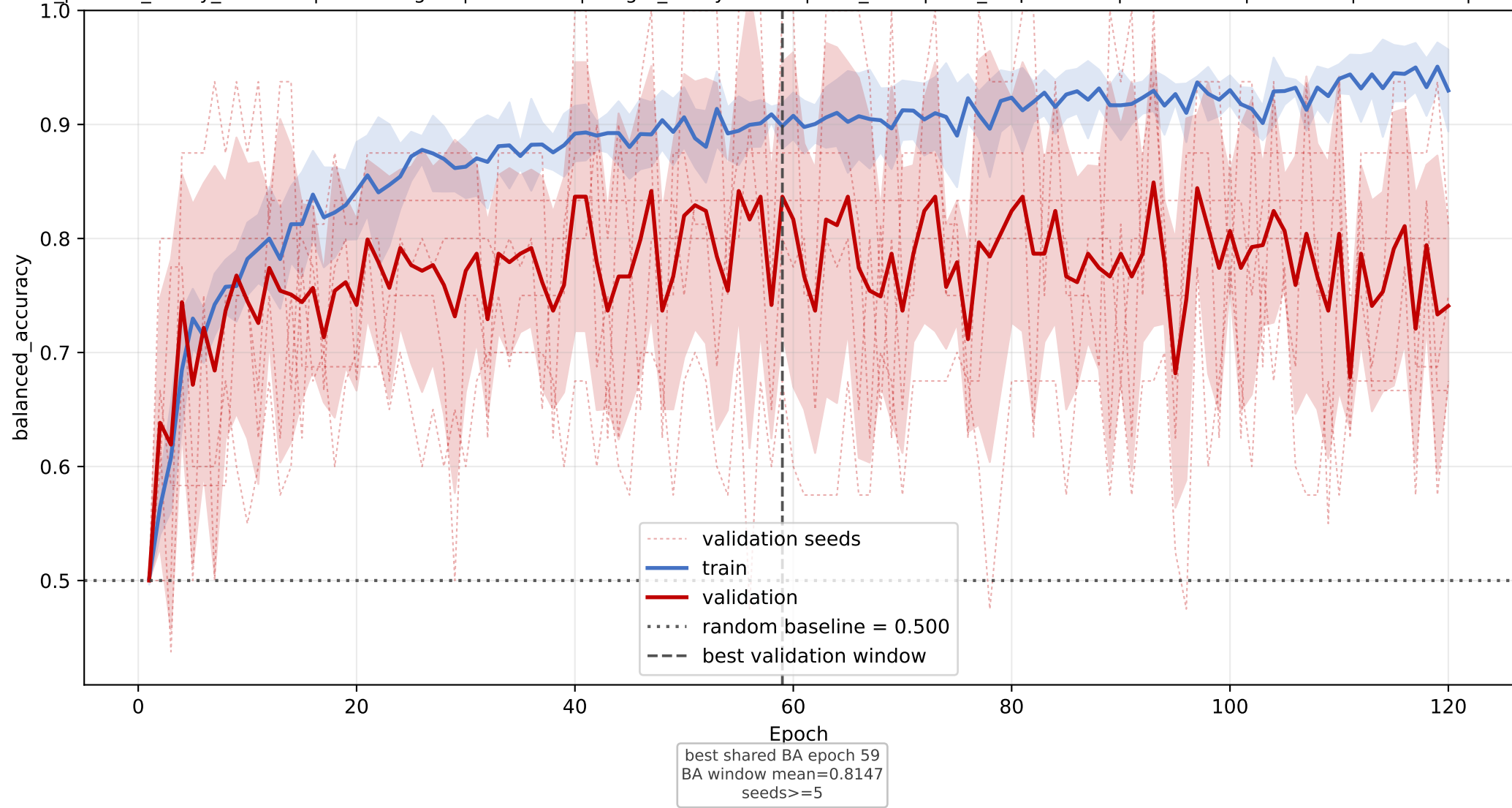
scp2: mean balanced_accuracy learning curve across seeds
