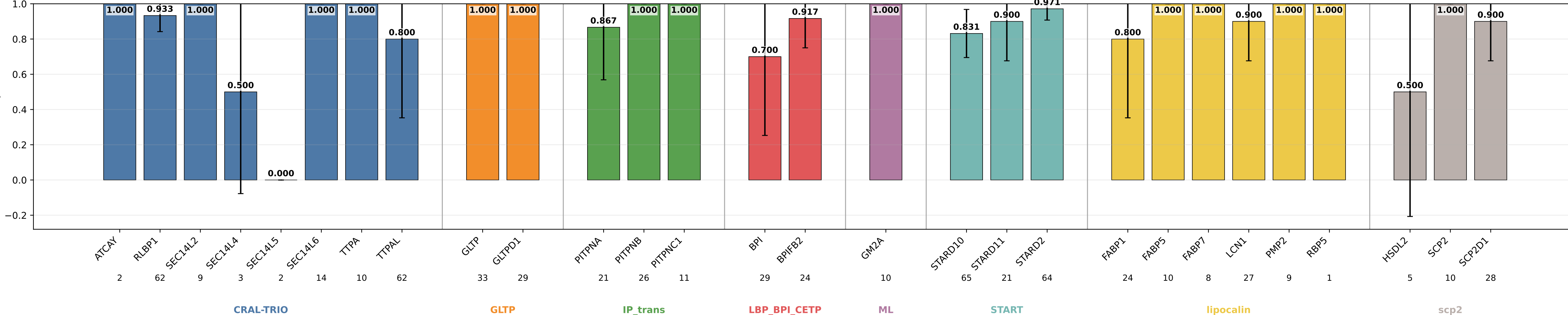
structural_pretrain_family_unfrozen sensitivity by subgroup structural_pretrain_family_unfrozen | class weights | lr=0.0001 | weight_decay=0.001 | final_m=4 | final_dropout=0.1 | hiddim=64 | heads=8 | batch=16 | ep=120 | seeds=0,1,2,3,4
