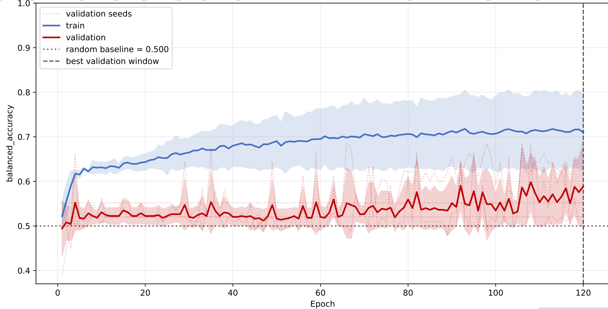
LBP_BPI_CETP: mean balanced_accuracy learning curve across seeds
