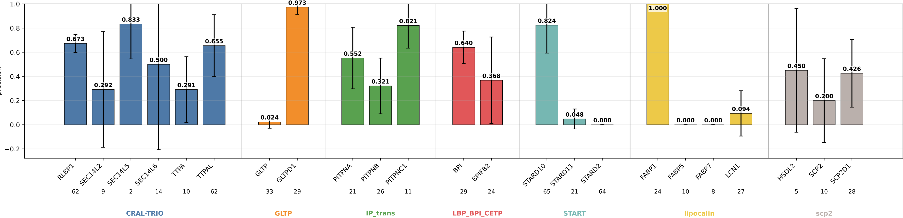
geometric_edge_mlp_protgeom_family_neutral_normalized_bilinear_fusion_bilinear_norm_bilinear_wd01 precision by subgroup geometric_edge_mlp_protgeom_family_neutral_normalized_bilinear_fusion_bilinear_norm_bilinear_wd01 | class weights | lr=0.0001 | weight_decay=0.01 | final_m=4 | final_dropout=0.1 | hiddim=8 | heads=8 | batch=16 | ep=120 | seeds=0,1,2,3,4
