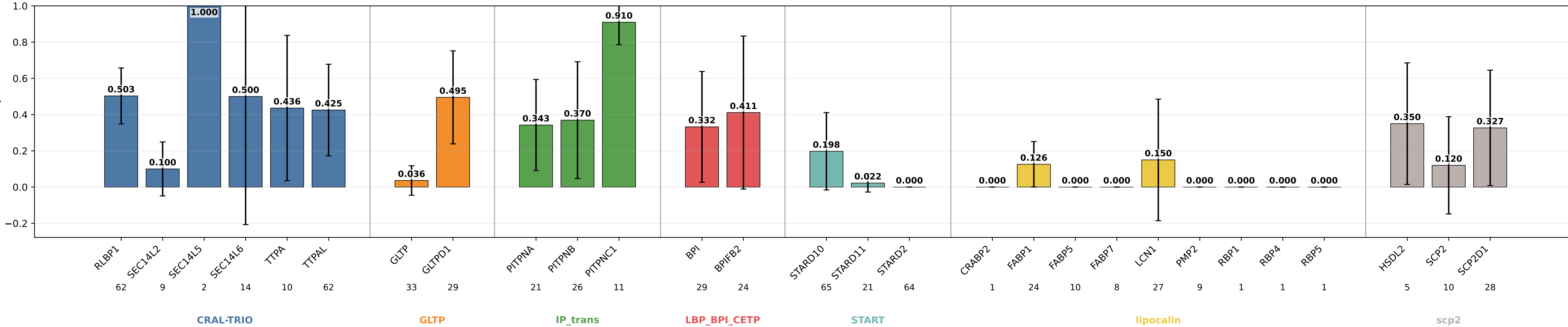
geometric_edge_mlp_protgeom_family_neutral_normalized_bilinear_fusion_bilinear_norm_bilinear_wd01 sensitivity by subgroup geometric_edge_mlp_protgeom_family_neutral_normalized_bilinear_fusion_bilinear_norm_bilinear_wd01 | class weights | lr=0.0001 | weight_decay=0.01 | final_m=4 | final_dropout=0.1 | hiddim=8 | heads=8 | batch=16 | ep=120 | seeds=0,1,2,3,4
