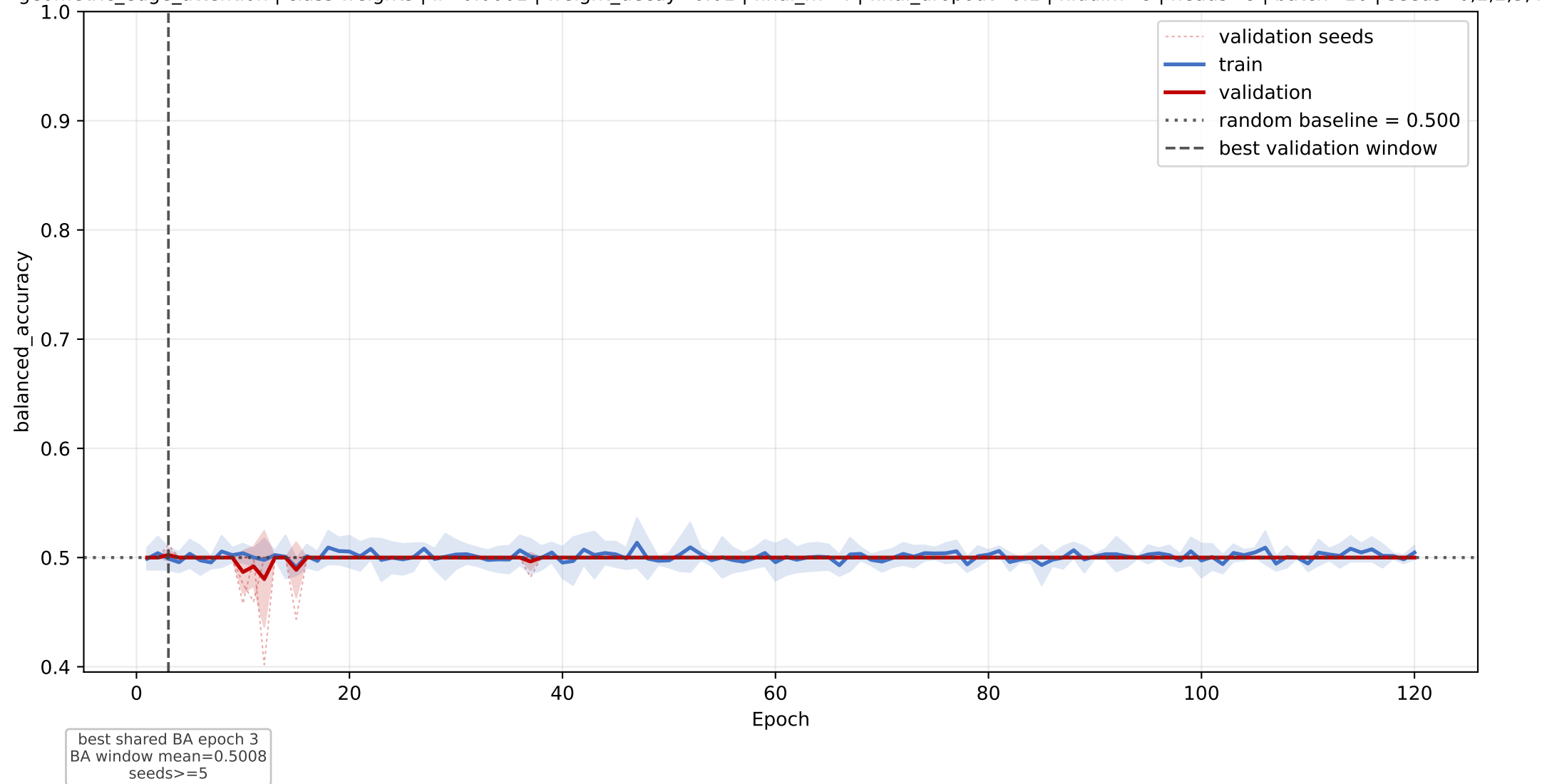
CRAL-TRIO: mean balanced_accuracy learning curve across seeds
