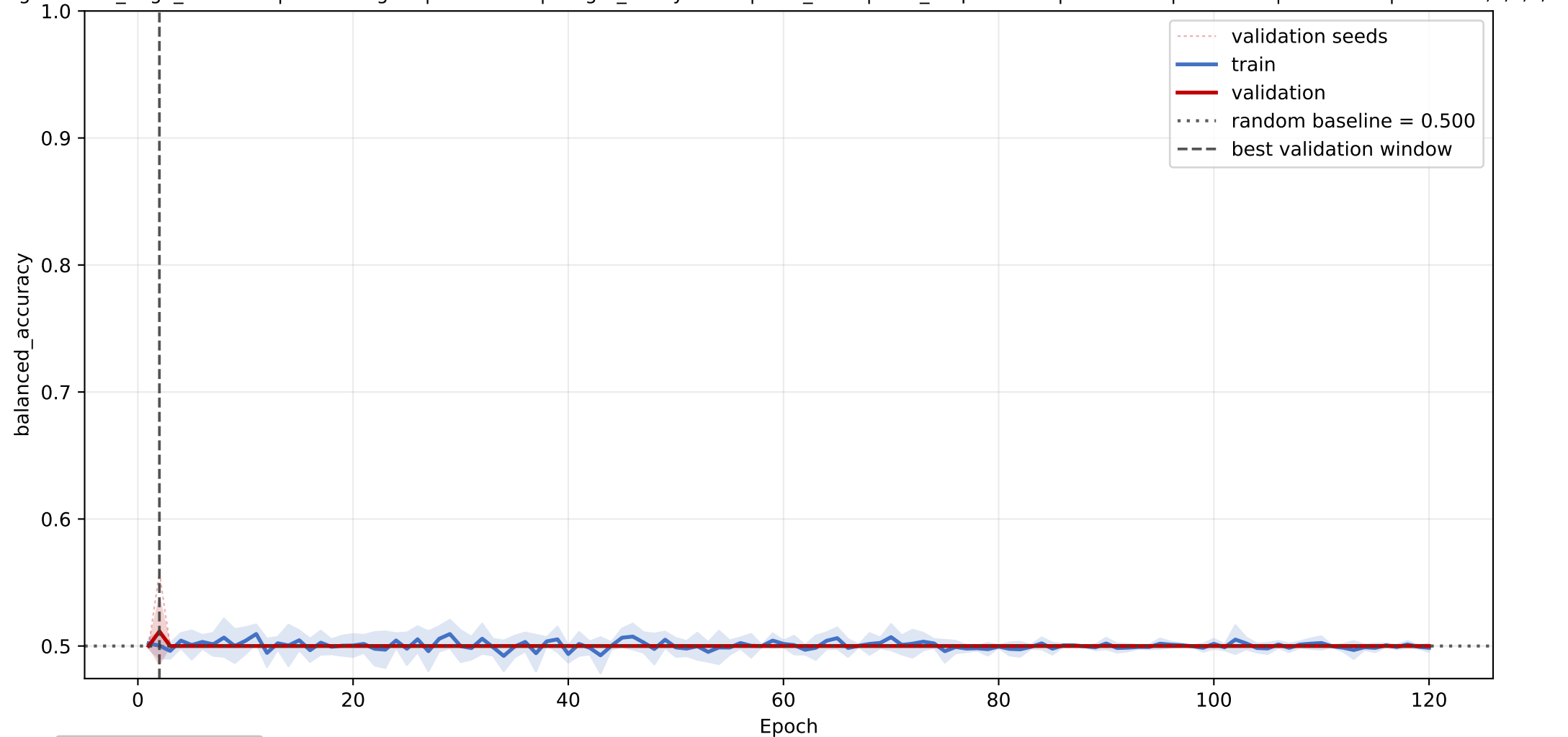
GLTP: mean balanced_accuracy learning curve across seeds
