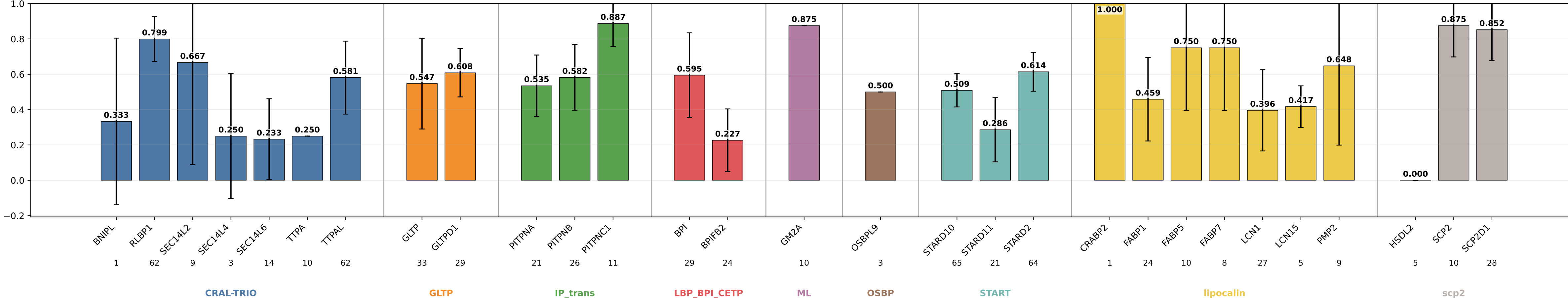
dh_s15_mbw_hid32_dpt0 AUC by subgroup dh_s15_mbw_hid32_dpt0 | class weights | lr=0.0001 | weight_decay=0.01 | final_m=4 | final_dropout=0.0 | hiddim=32 | heads=8 | batch=16 | ep=120 | seeds=0,1,2,3,4
