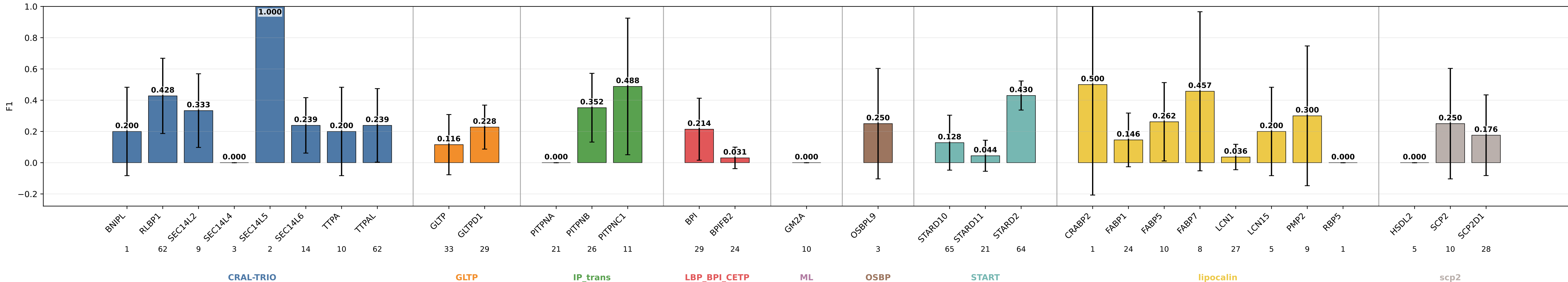
dh_s15_mbw_hid32_wd1e5 F1 by subgroup dh_s15_mbw_hid32_wd1e5 | class weights | lr=0.0001 | weight_decay=1e-05 | final_m=4 | final_dropout=0.1 | hiddim=32 | heads=8 | batch=16 | ep=120 | seeds=0,1,2,3,4
